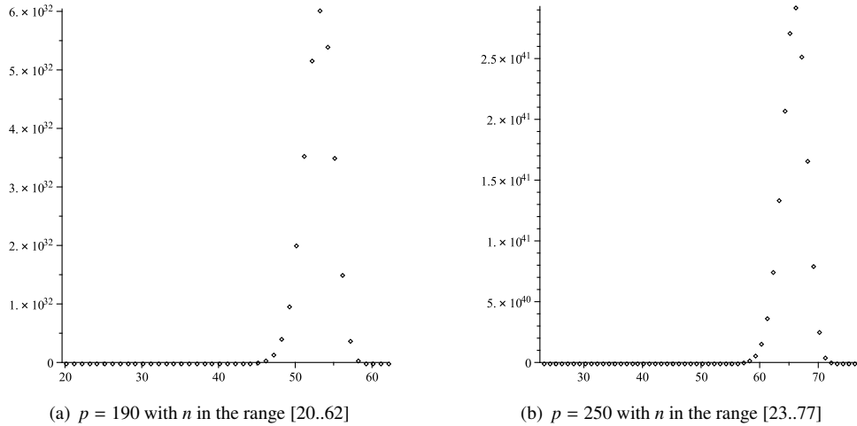
Figure 3: Plots of g(n, p)
