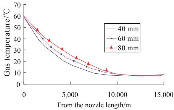
Figure 11 The Dropping of Temperature of Different Thickness of Thermal Conductivity Along the Pipe
