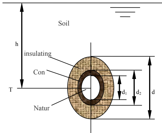
Figure 1 Schematic Diagram of Buried Gas Pipeline
