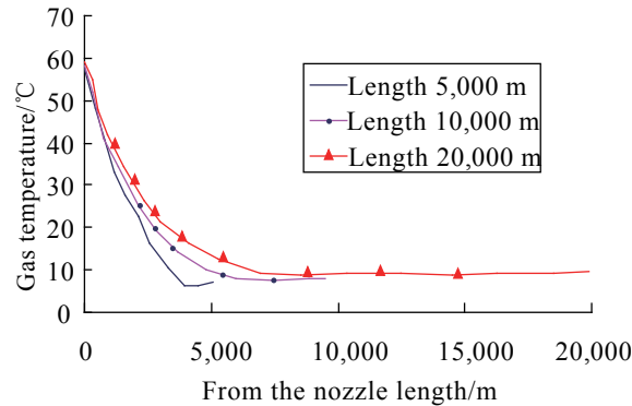
Figure 6 The Dropping of Temperature of Different Length Along the Pipe
