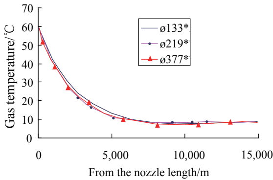
Figure 5 The Dropping of Temperature of Different Diameter Along the Pipe
