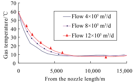
Figure 7 The Dropping of Temperature of Different Flow Along the Pipe
