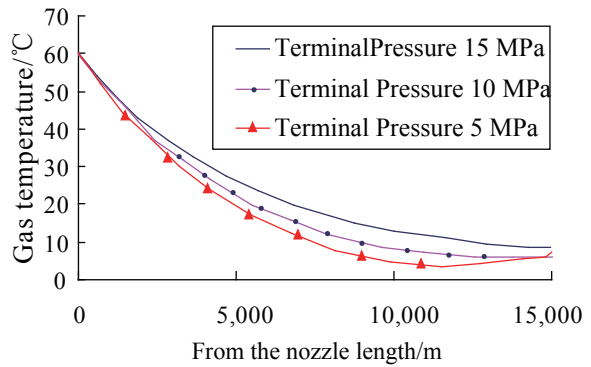
Figure 9 The Dropping of Temperature of Different Ending Pressure Along the Pipe
