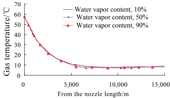
Figure 4 The Dropping of Temperature of Different Content of Water Vapor Along the Pipe
