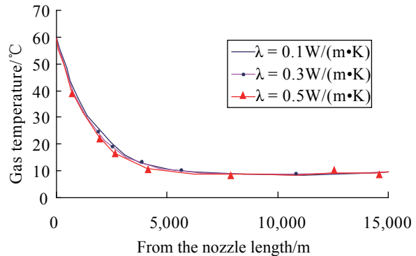
Figure 10 The Dropping of Temperature of Different Thermal Conductivity of the Insulation Layer Along the Pipe
