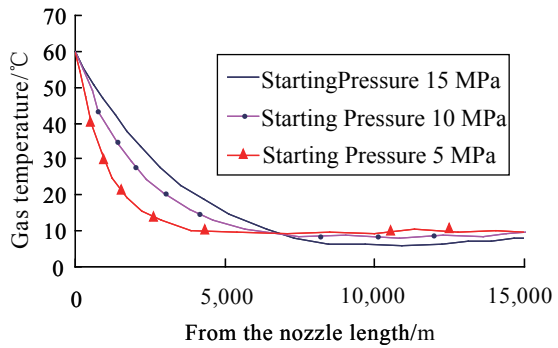
Figure 8 The Dropping of Temperature of Different Starting Pressure Along the Pipe
