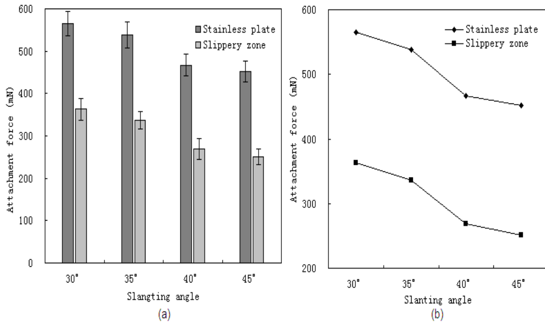
Fig. 4: Maximal attachment force generated by locusts on slippery zone and stainless steel plate with different slanting angles. (a) Presenting the maximal values. (b) Exhibiting the decreasing trend.
